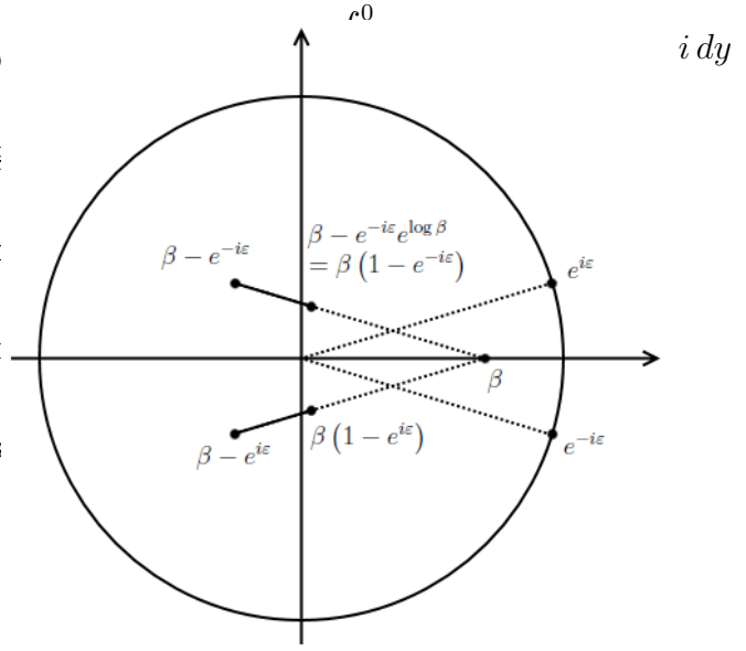
Figure 2: Points \beta - e^{iz} for z \in I_1 and z \in I_5 .
